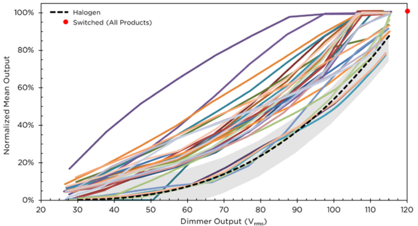
● Figuur 3: dim-curves van 31 dimbare LED lampen (bron: DoE)
